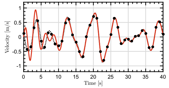
Fig. 6 Comparison between the time-domain output of the reduced order model \hat{\mathcal{H}}_{(1,1,8,2,3)} (solid-red) and the force-to-velocity frequency response \mathcal{H} (dotted-black).
