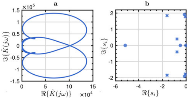
Fig. 8 Pole-zero map of the moment-matching parametric model of the radiation force kernel \tilde{K}_{(0.8,1.75,2.6)}(j\omega)
