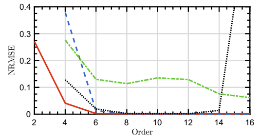
Fig. 11 The NRMSE of the time-domain output computed using a moment-matching force-to-velocity approximated model (solid-red), and using the approximated radiation impulse response computed using moment-matching (dashed-blue), NTNU method (dotted-black) and Prony's method (dash-dot-green) for different model orders.
